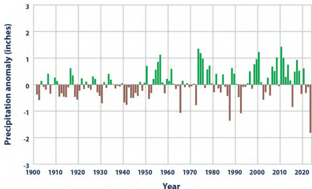
Figure 18. Precipitation Worldwide, 1901–2023
