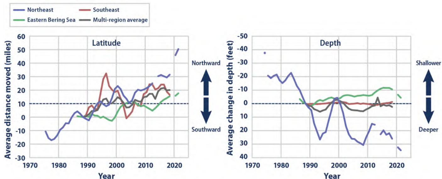
Figure 35. Change in Latitude and Depth of Marine Species, 1974–2022
