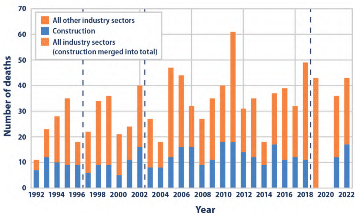
Figure 11. Heat-Related Workplace Deaths in the United States, 1992–2022
